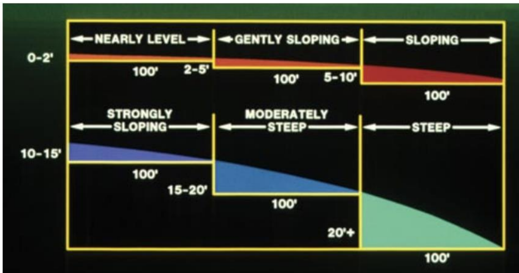
Figure 22.—Slope classes.
